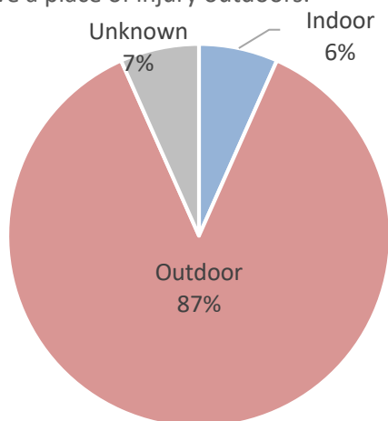
Graph 2. The majority of heat-associated deaths have a place of injury outdoors.
